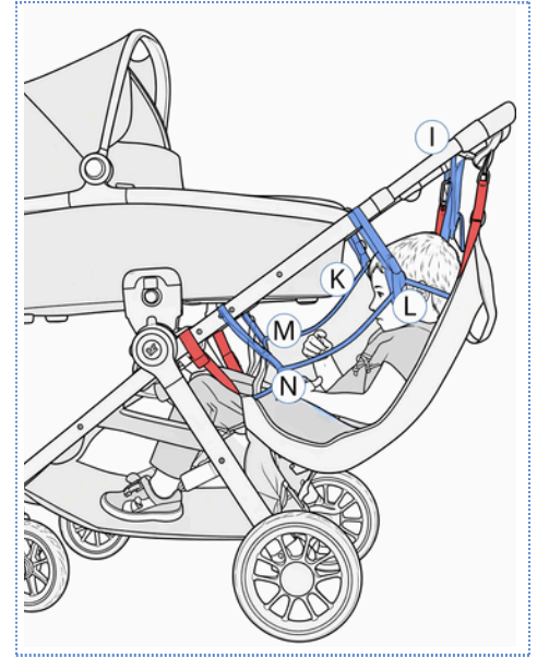
HEADBOARD STRAPS (I, J) AND PROTECTIVE WINGS (K, L, M, N) SIDE VIEW
